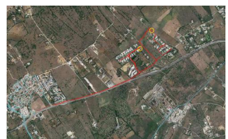
Ferrel
